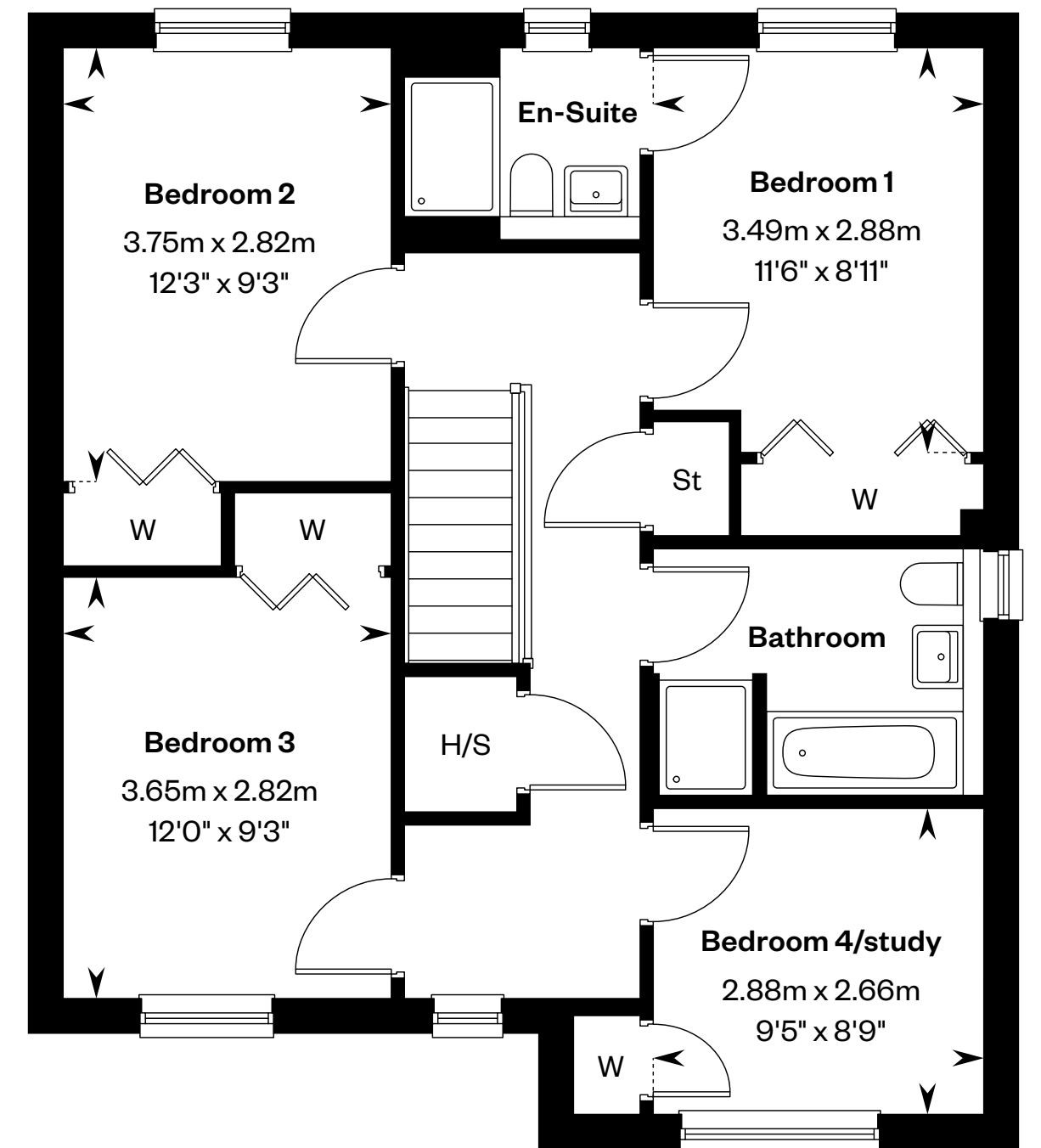
First floor
