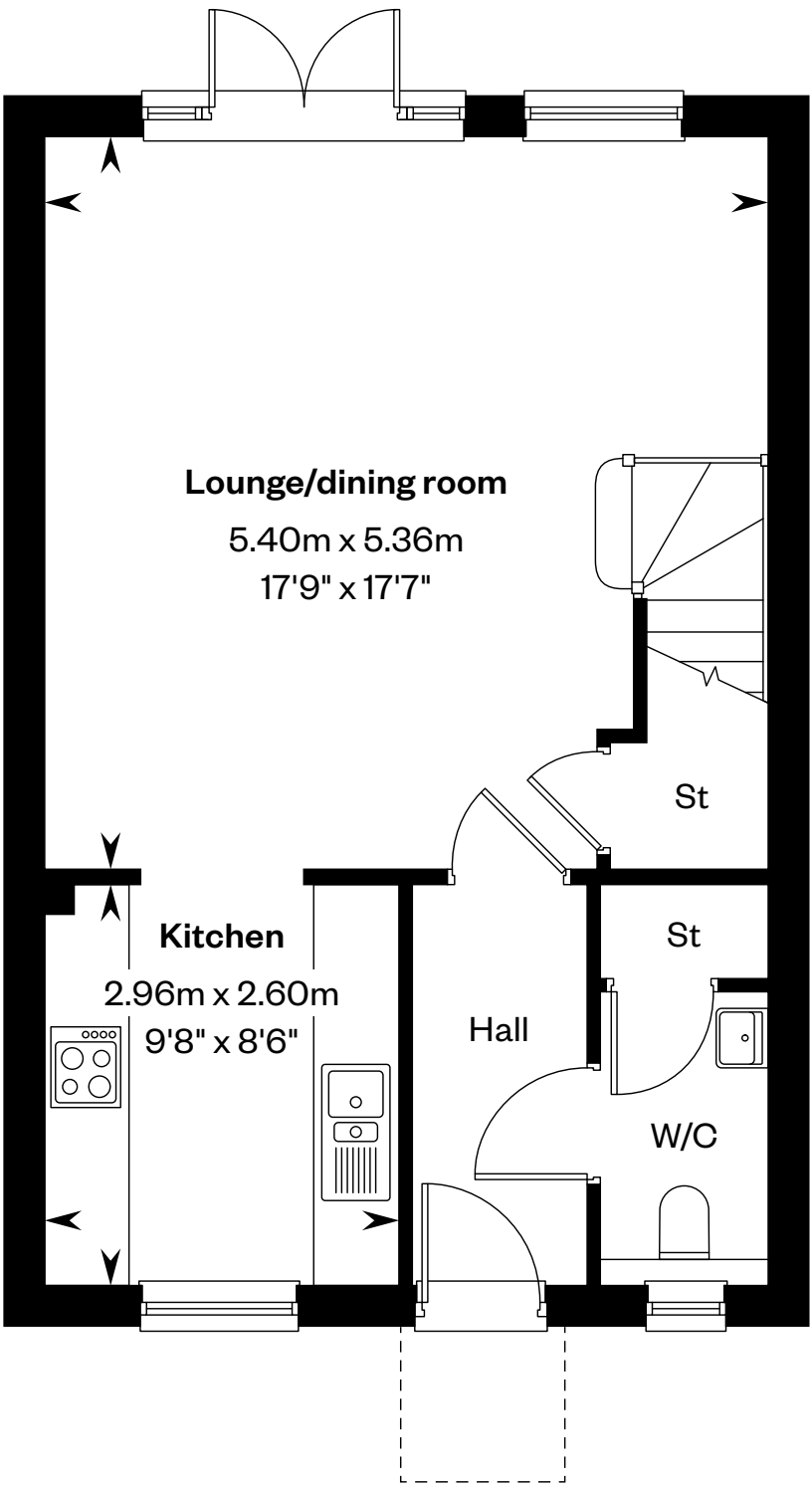
Ground floor
