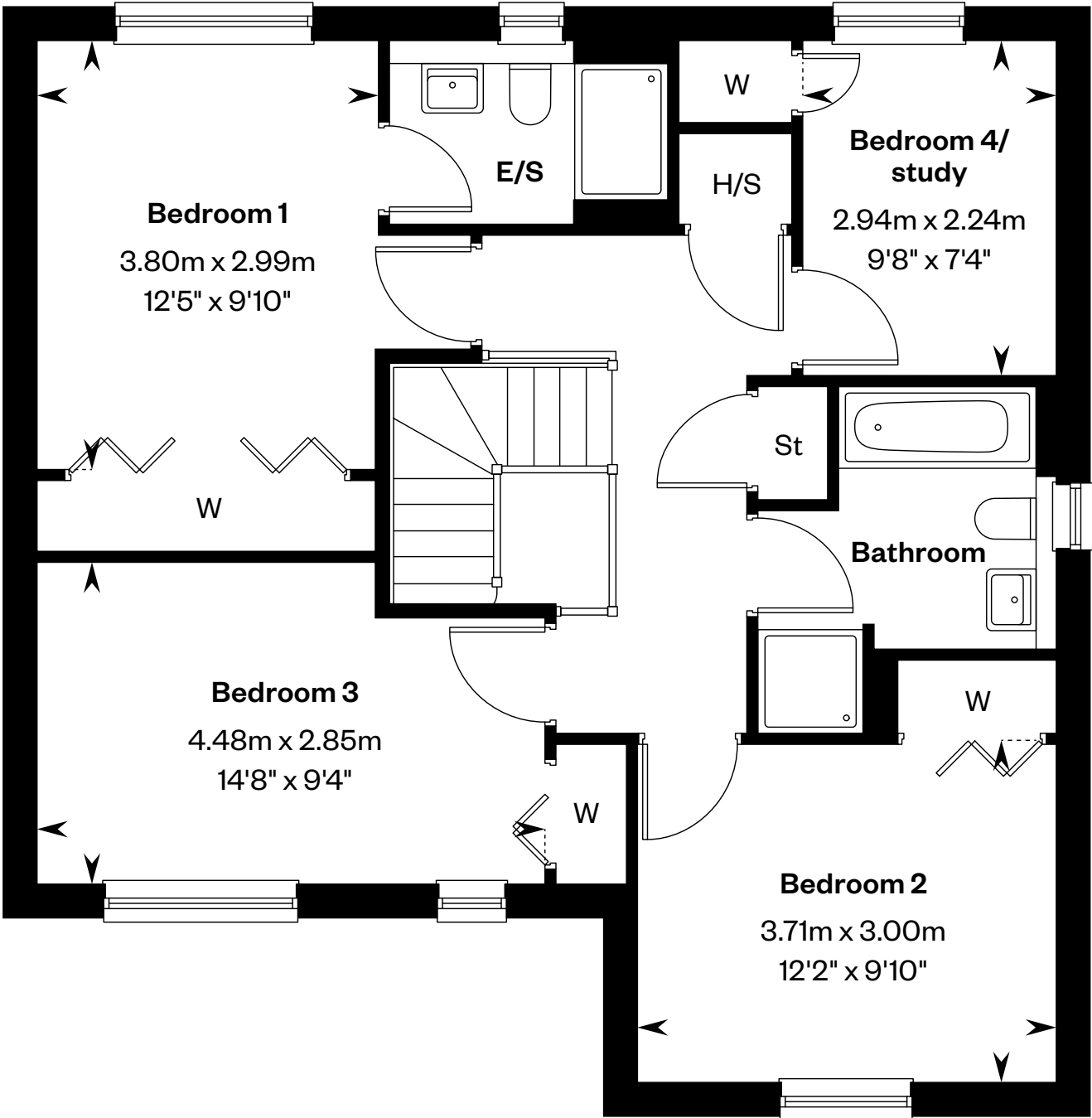
First floor
