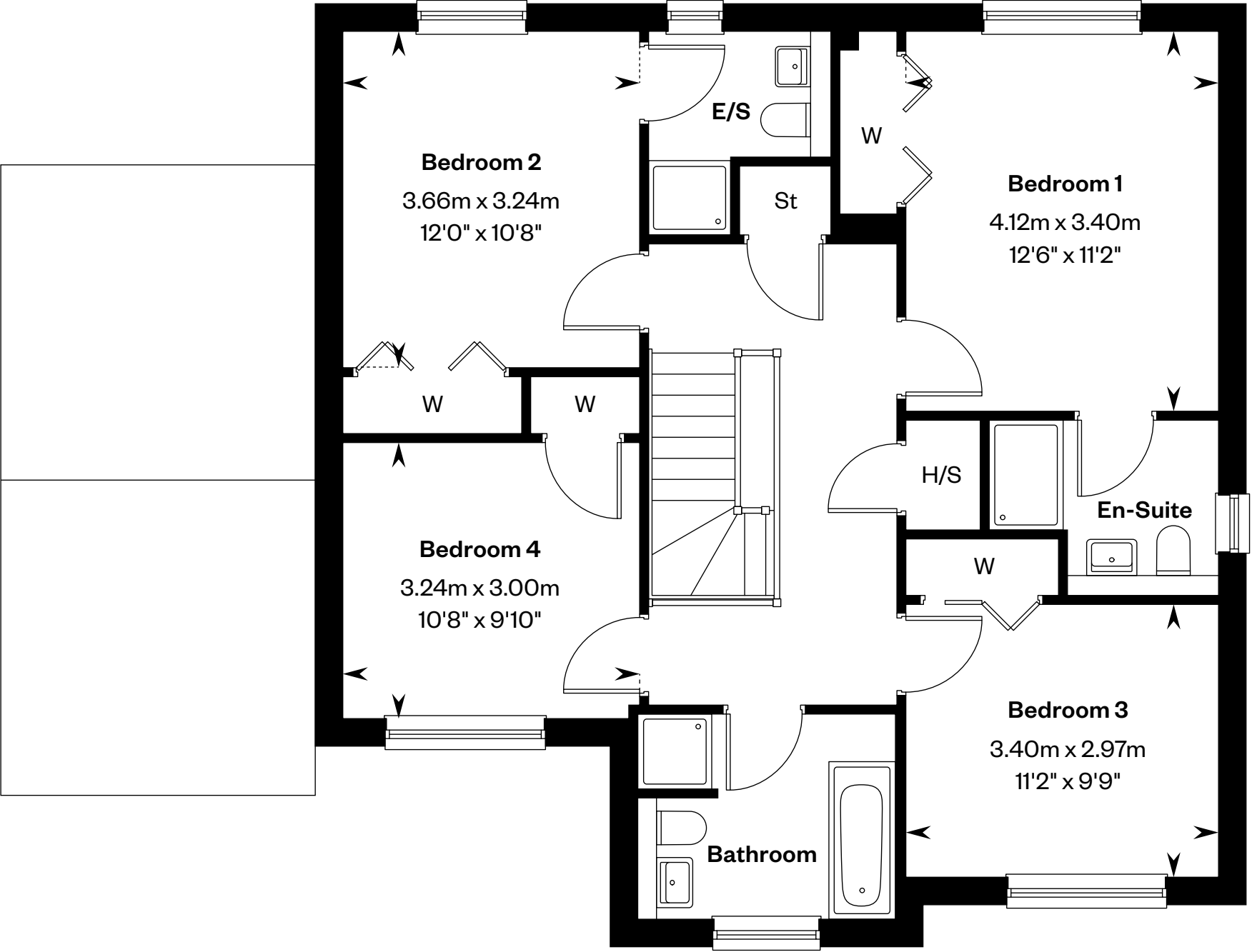
First floor
