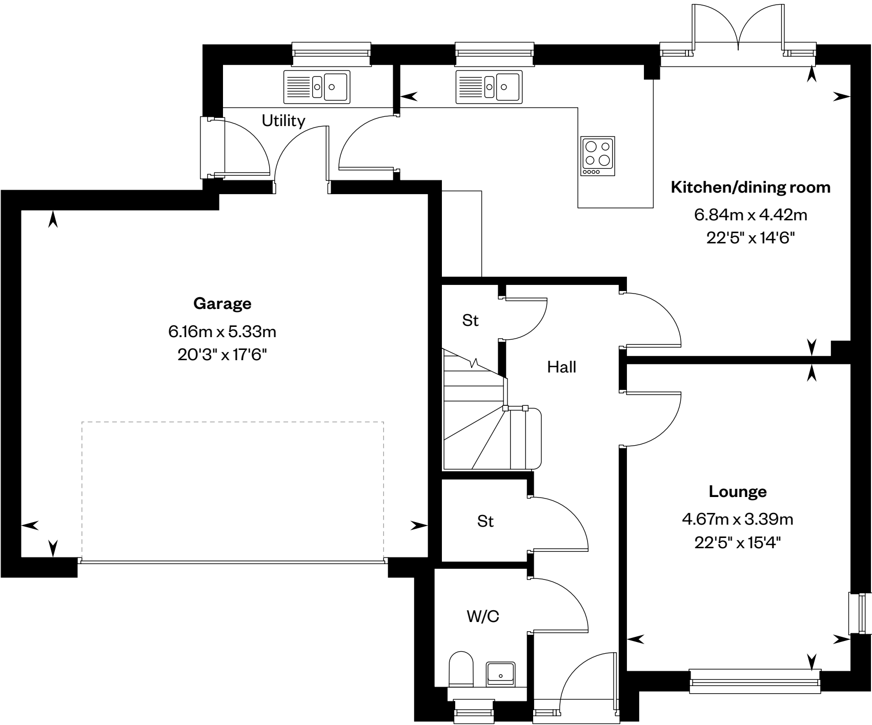
Ground floor
