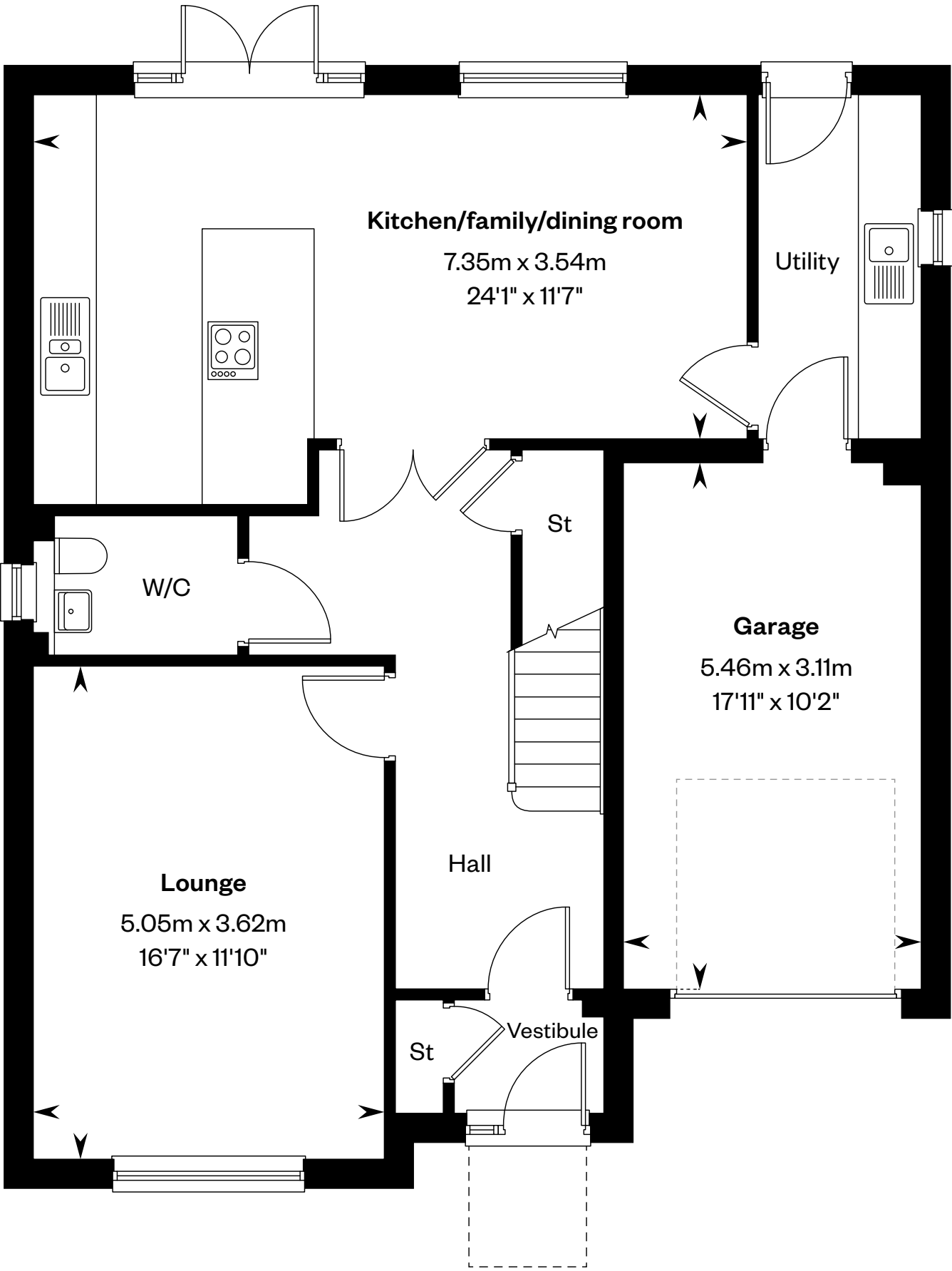
Ground floor
