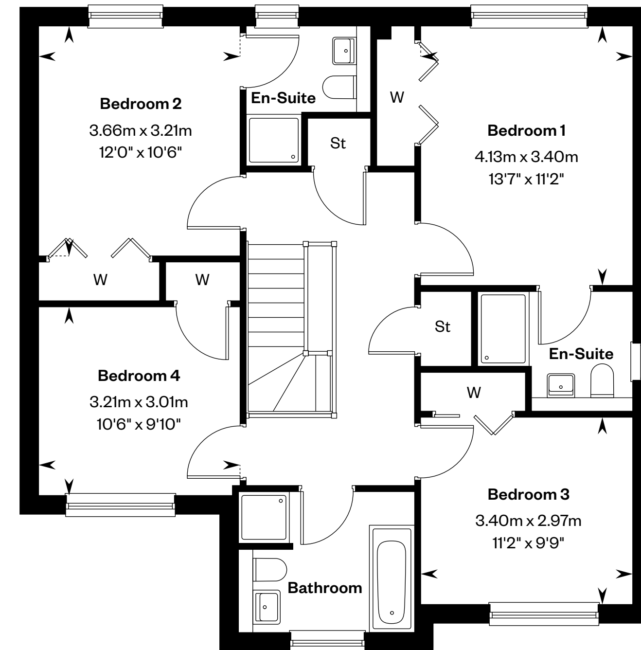
First floor
