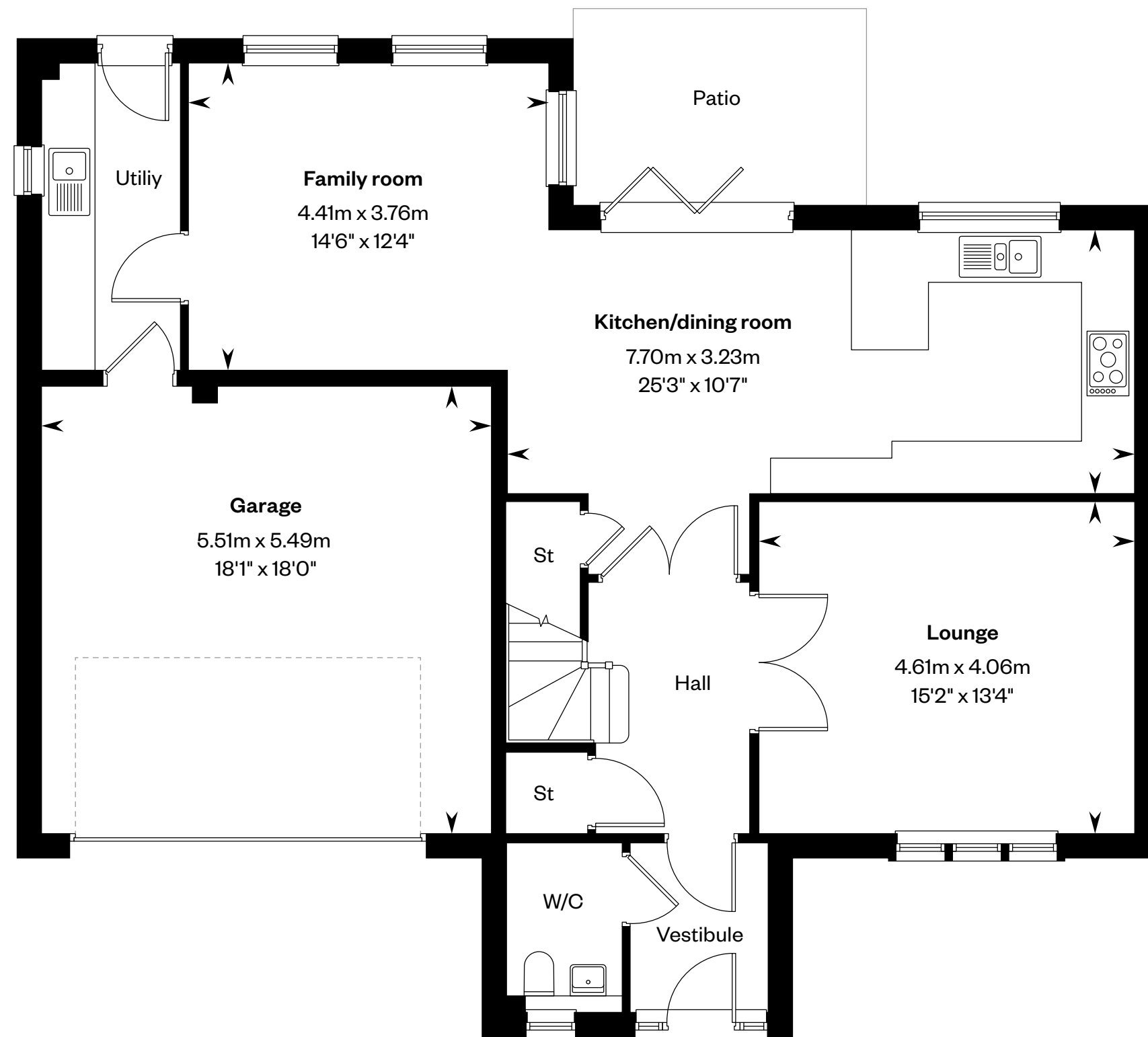
Ground floor
