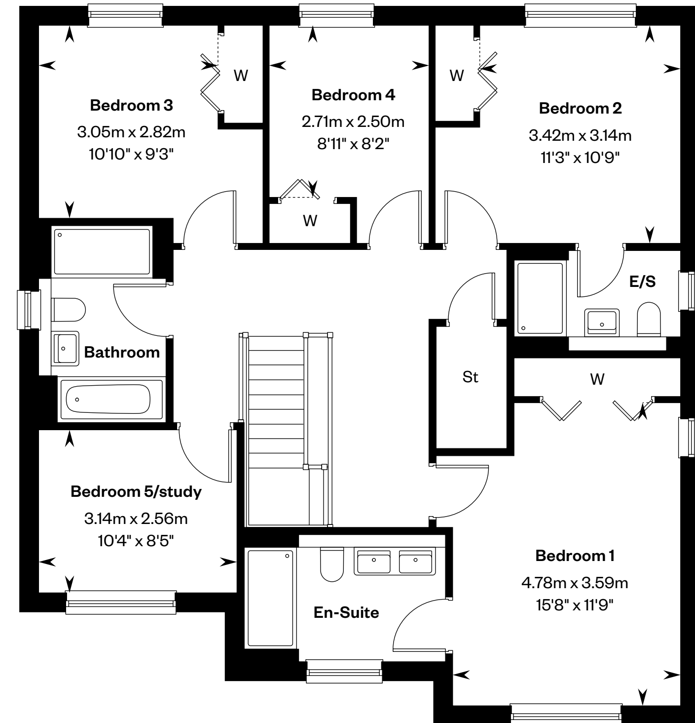
First floor
