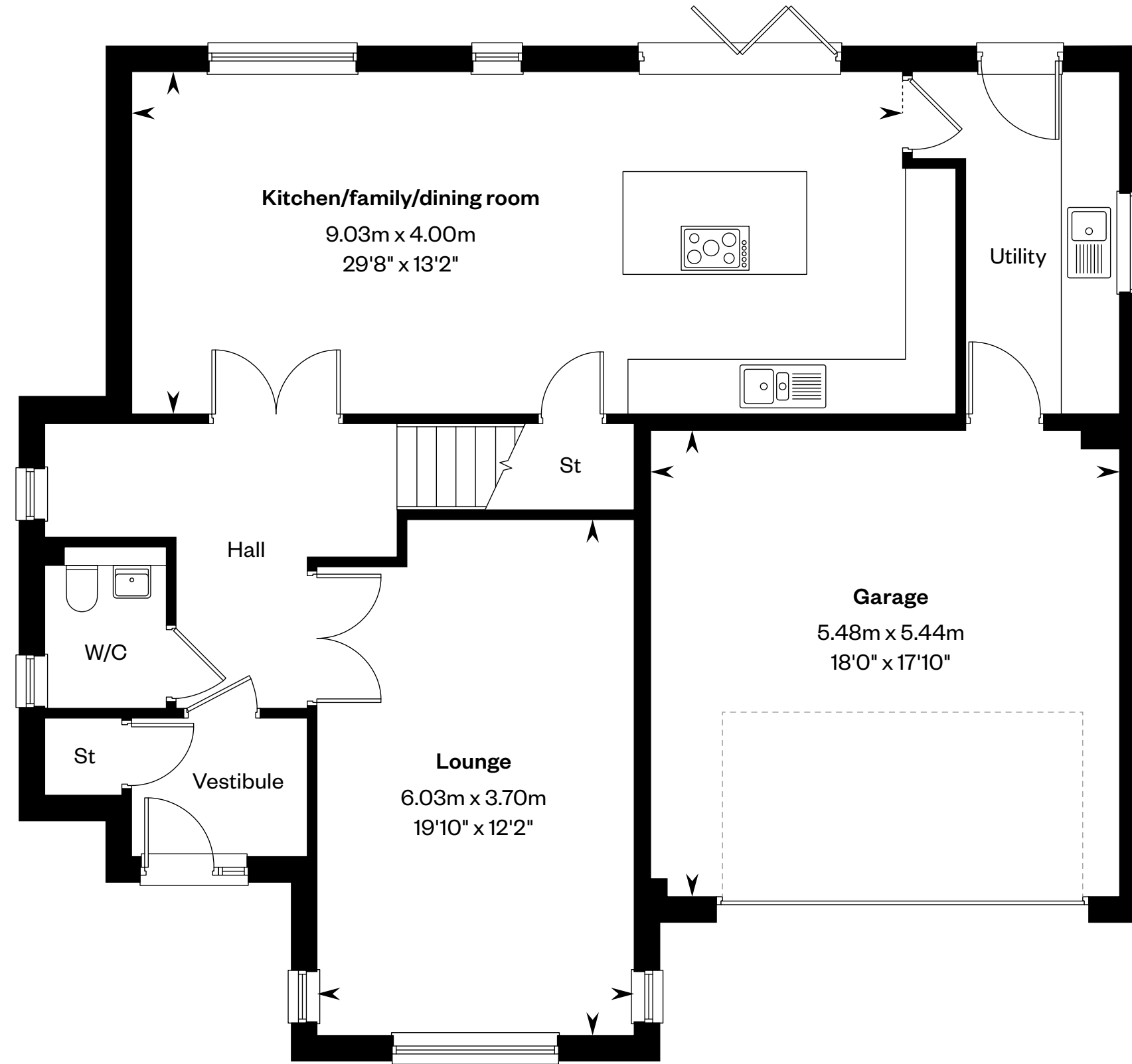
Ground floor
