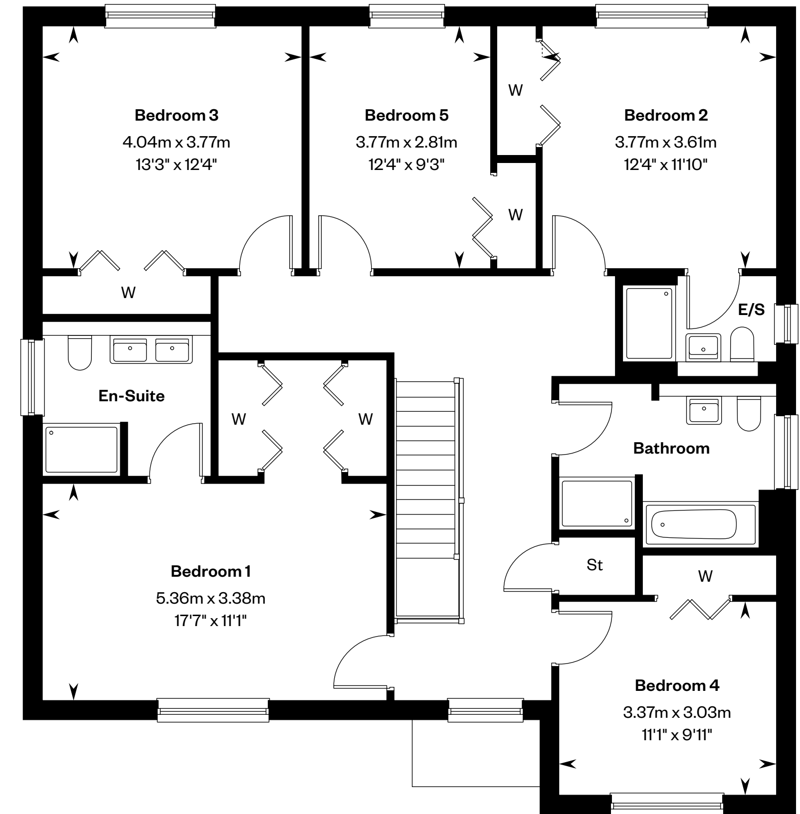
First floor
