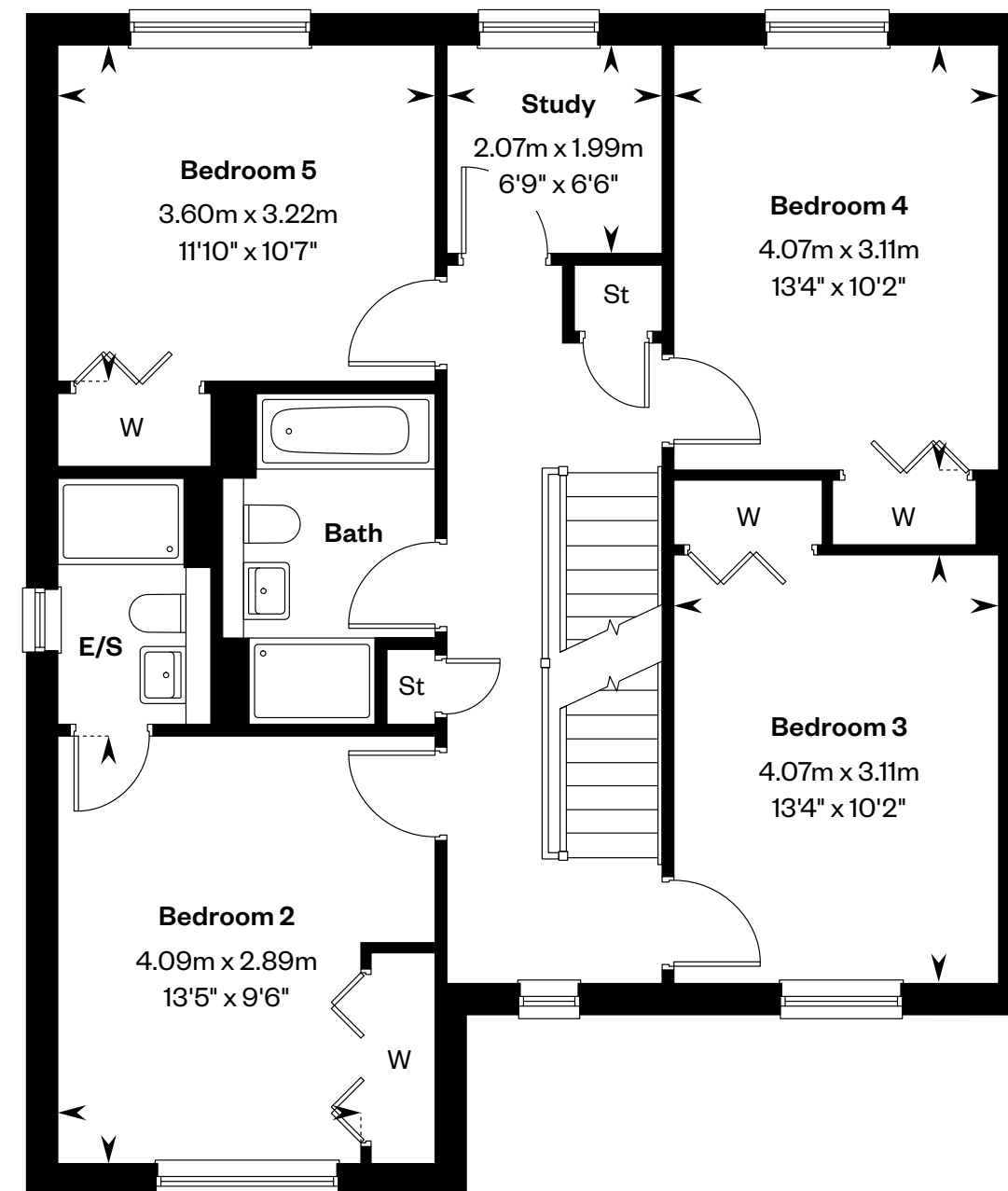
First floor
