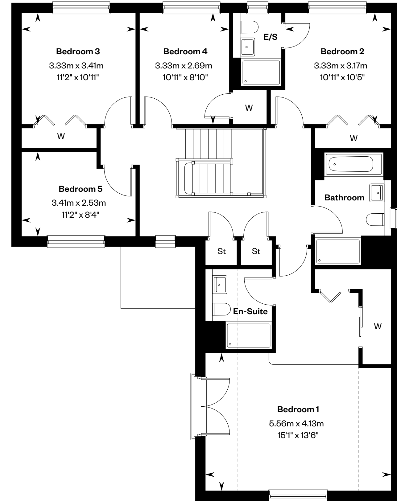
First floor
