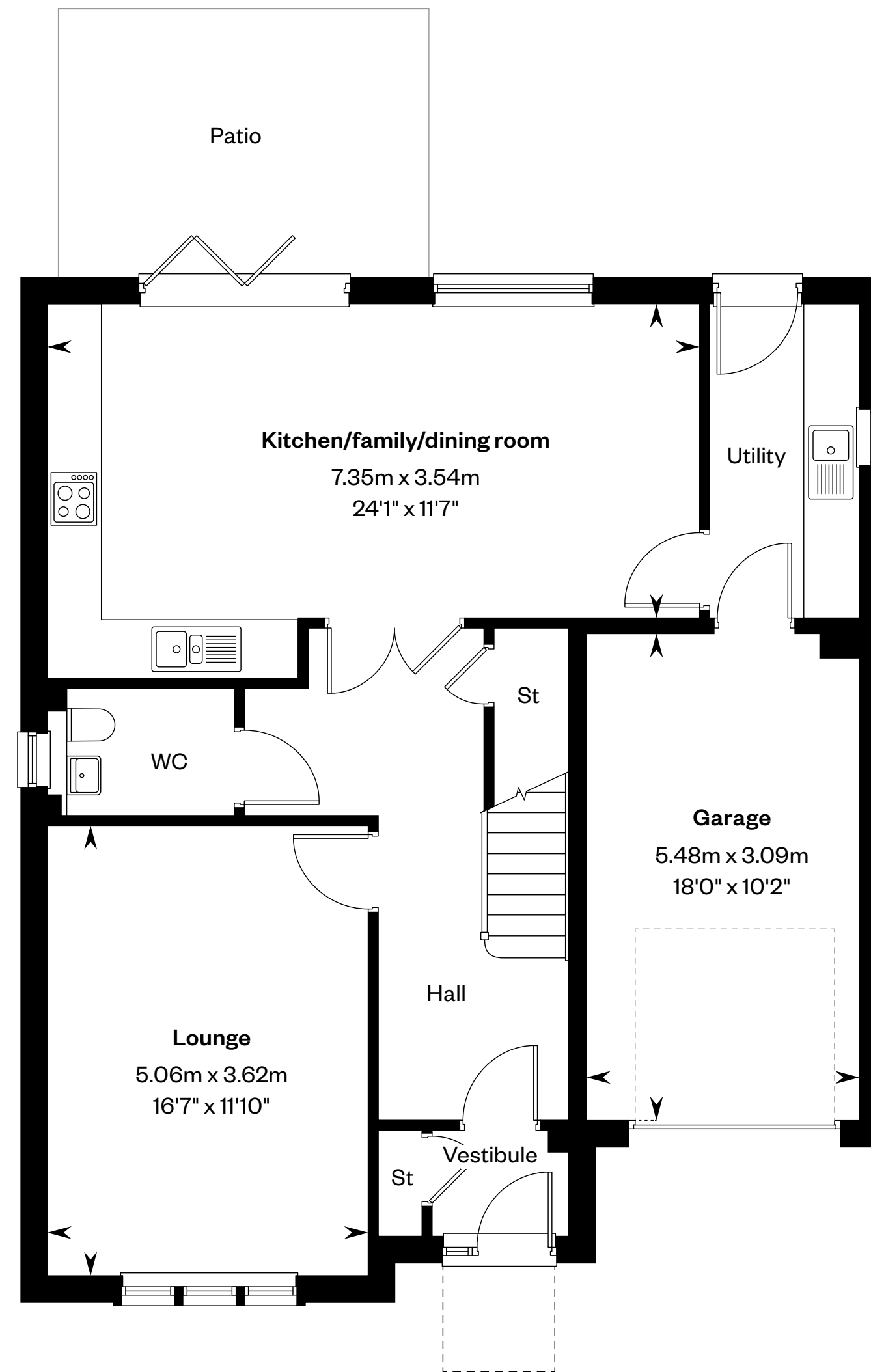
Ground floor
