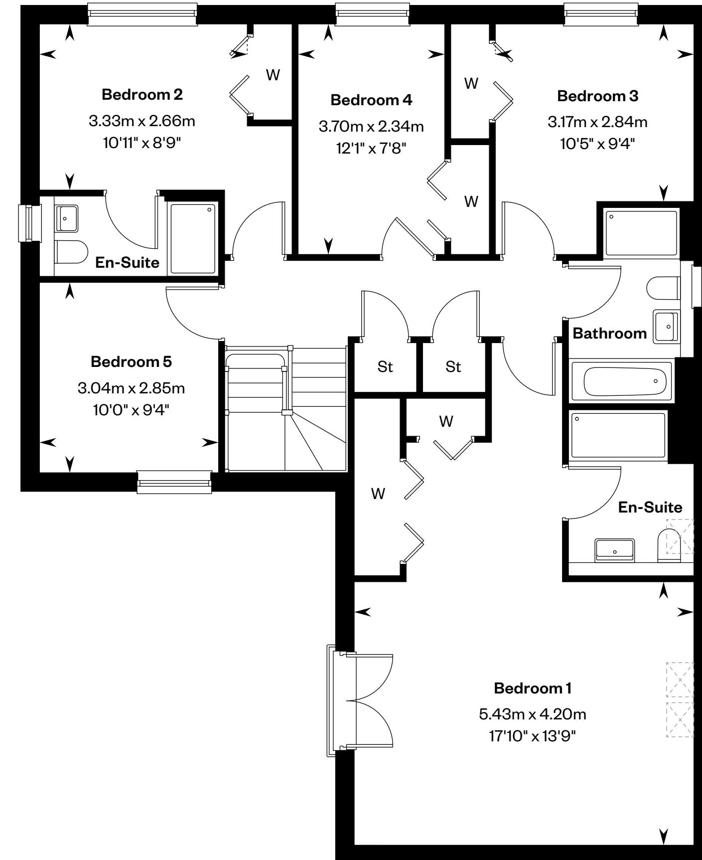
First floor
