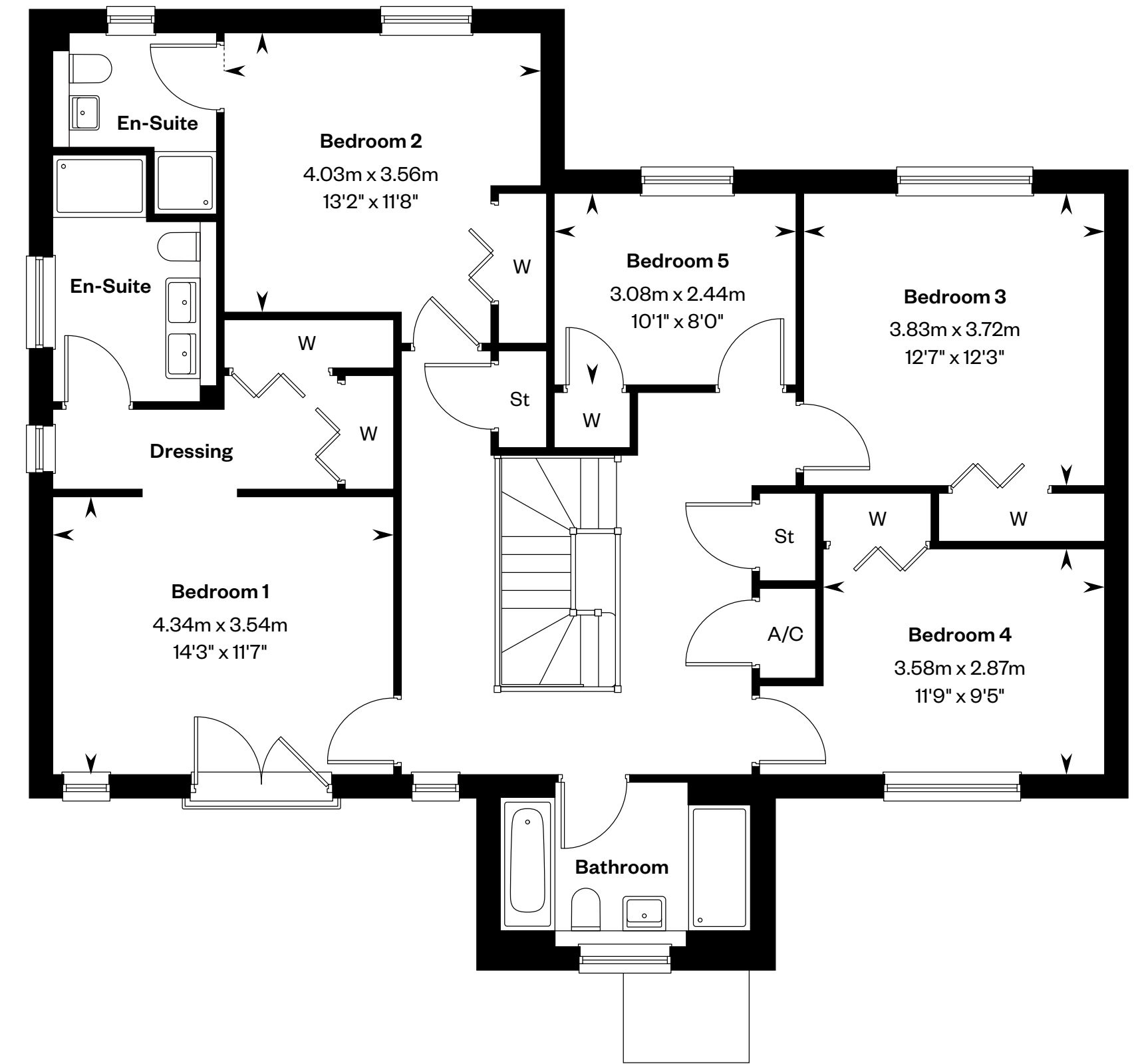
First floor
