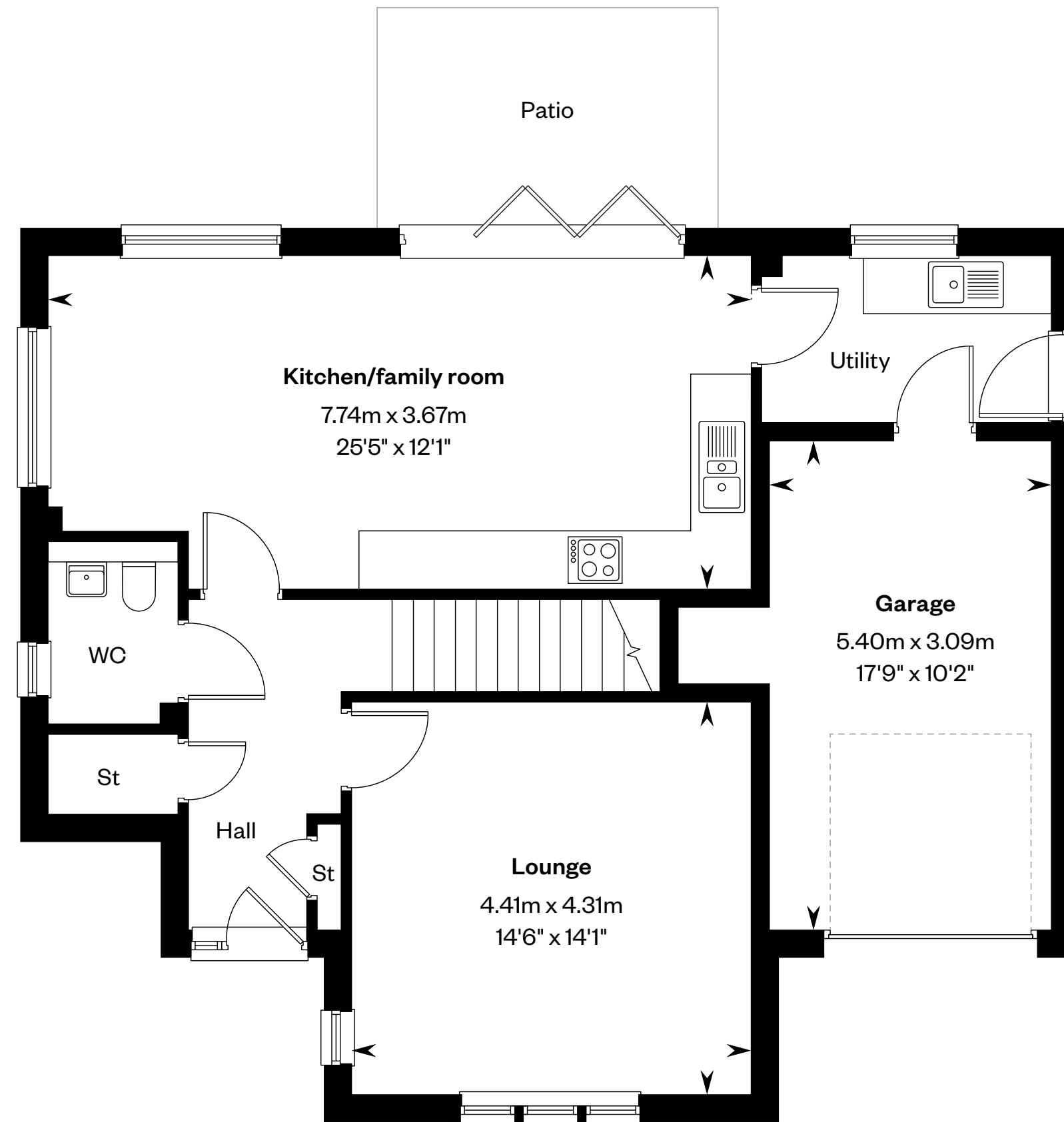
Ground floor
