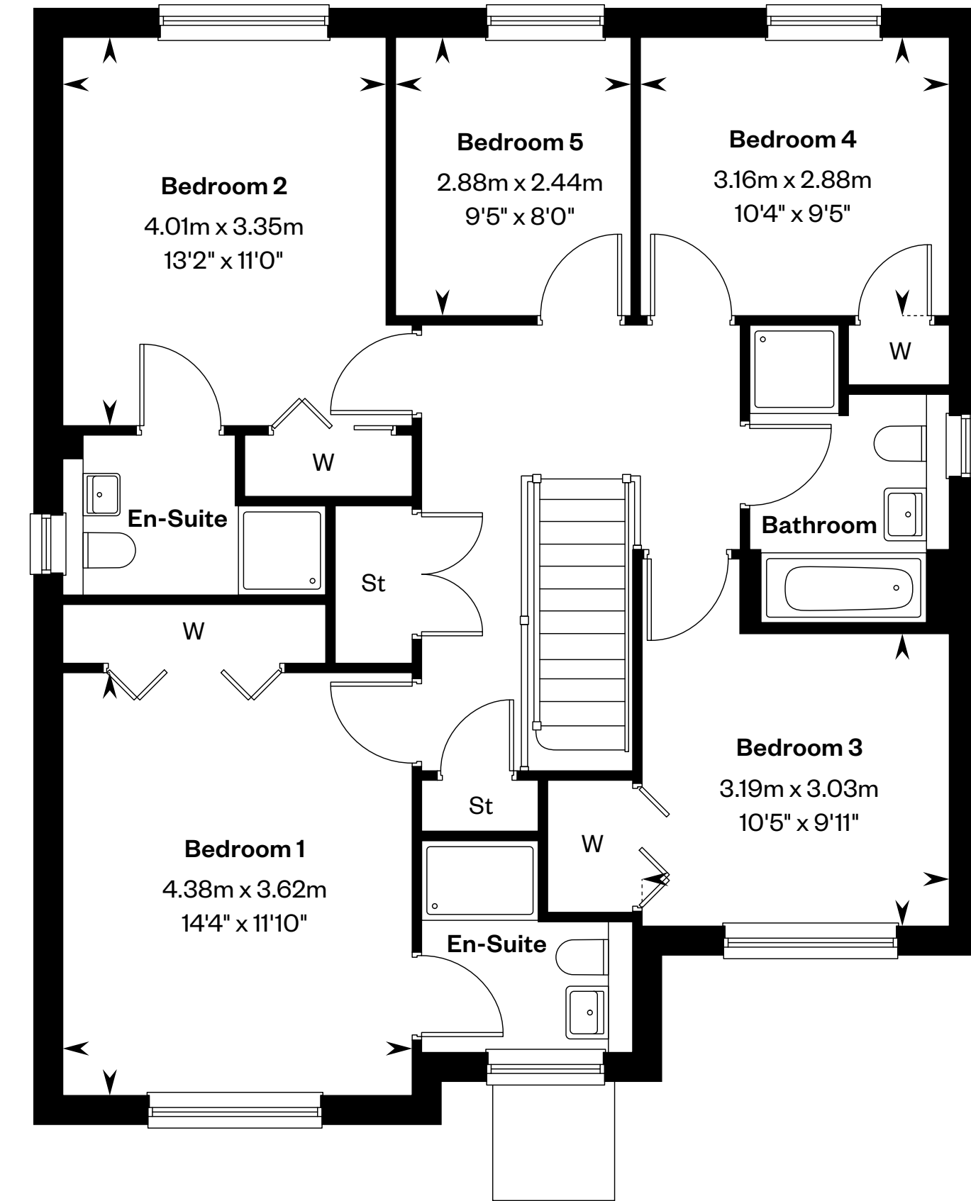
First floor
