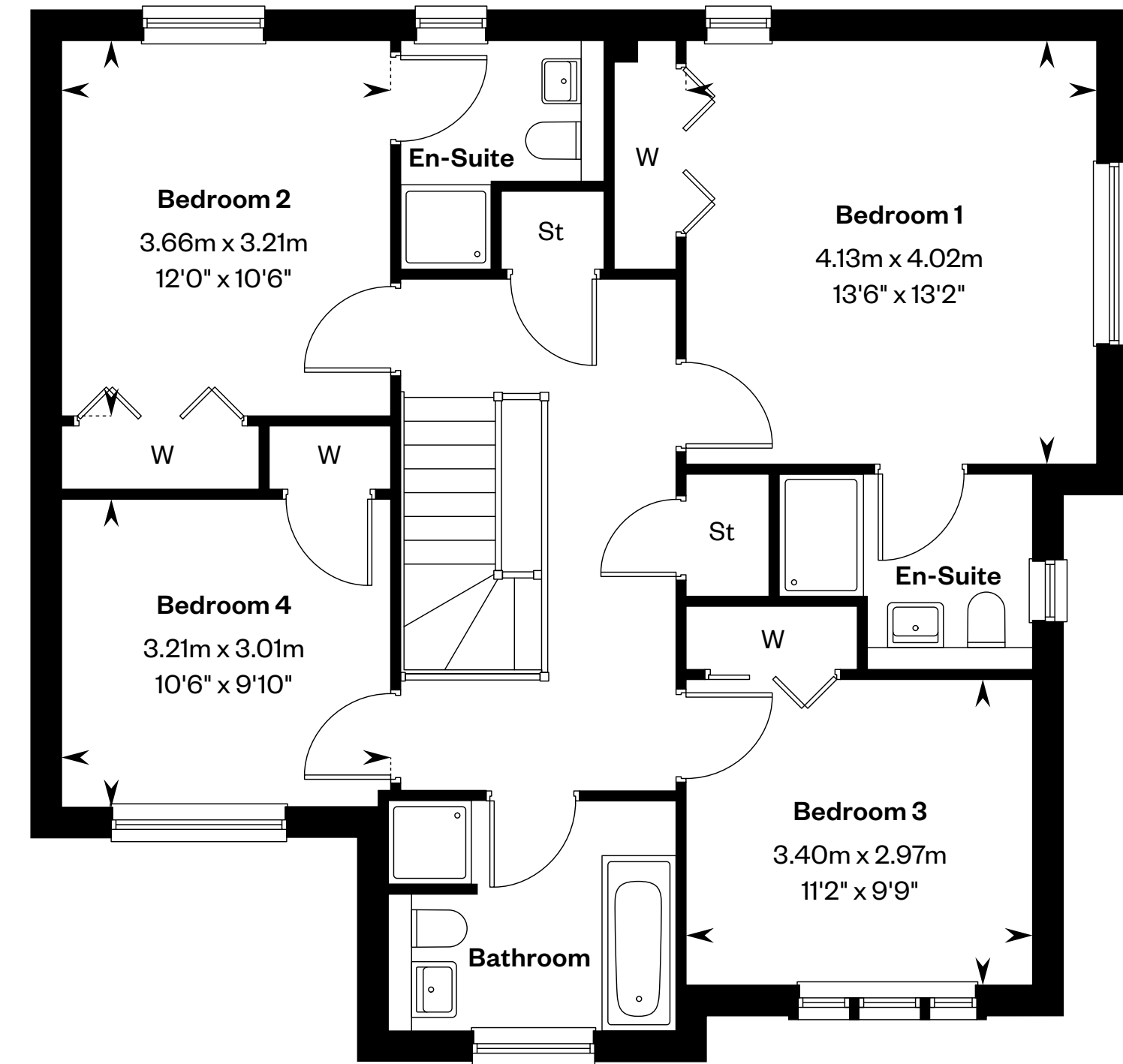
First floor
