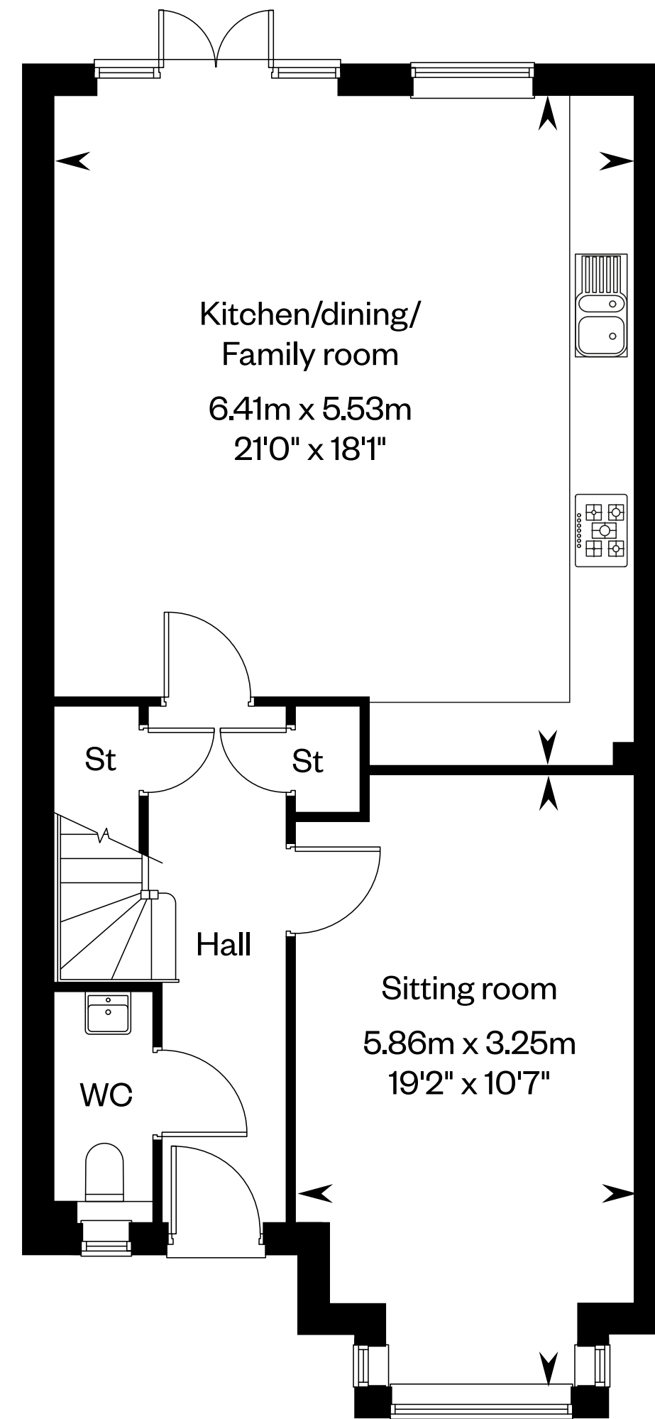
Ground floor
